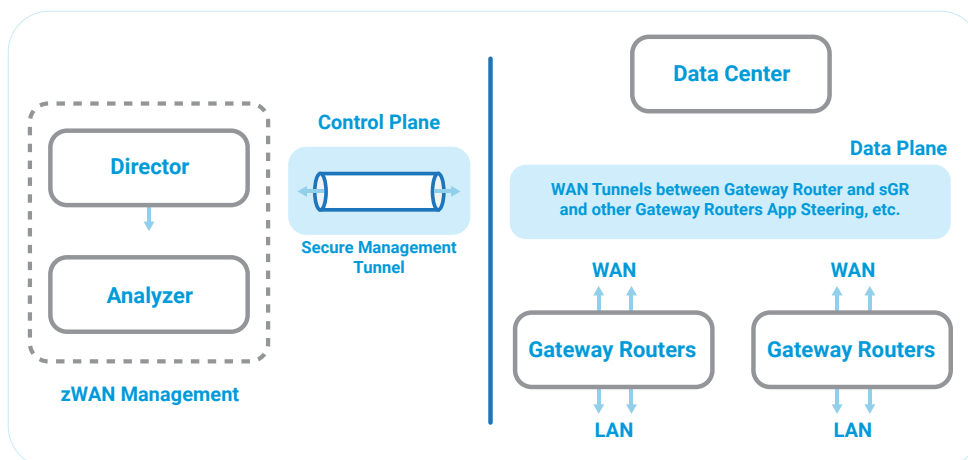
Figure 1: zWAN Architecture
